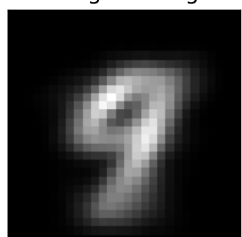
factor 3 \lambda=91.24 weighted avg
