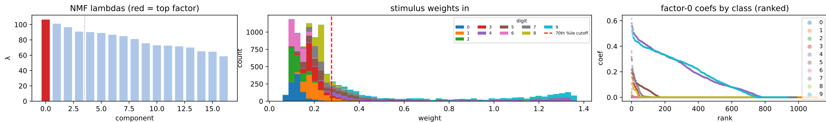
factor 0 \lambda=106.96 weighted avg
