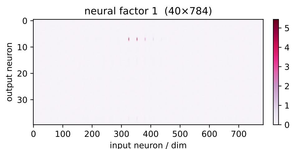
factor 1 \lambda=101.64 weighted avg
