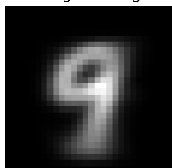
factor 2 \lambda=97.09 weighted avg
