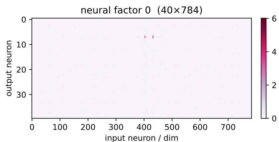
factor 0 \lambda=106.96 weighted avg
