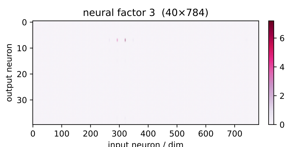
factor 3 \lambda=91.24 weighted avg
