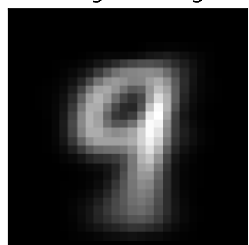
factor 1 \lambda=101.64 weighted avg
