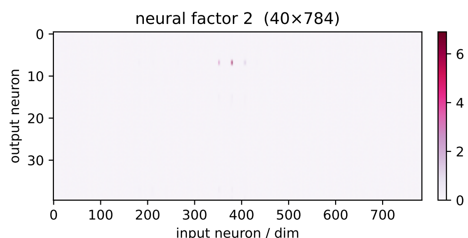
factor 2 \lambda=97.09 weighted avg
