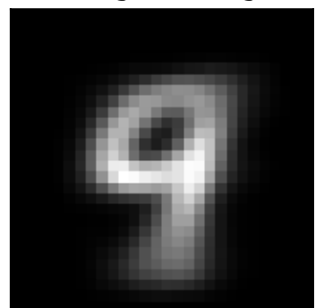
factor 0 \lambda=106.96 weighted avg
