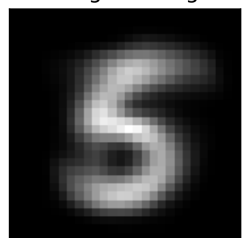
inh factor 0 \lambda=244.07 weighted avg
