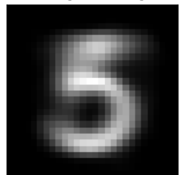
inh factor 3 \lambda=191.52 weighted avg
