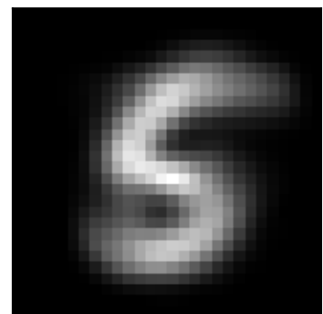
inh factor 1 \lambda=215.09 weighted avg
