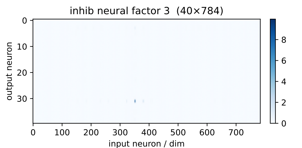
inh factor 3 \lambda=191.52 weighted avg
