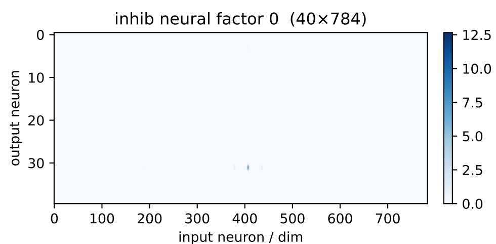
inh factor 0 \lambda=244.07 weighted avg
