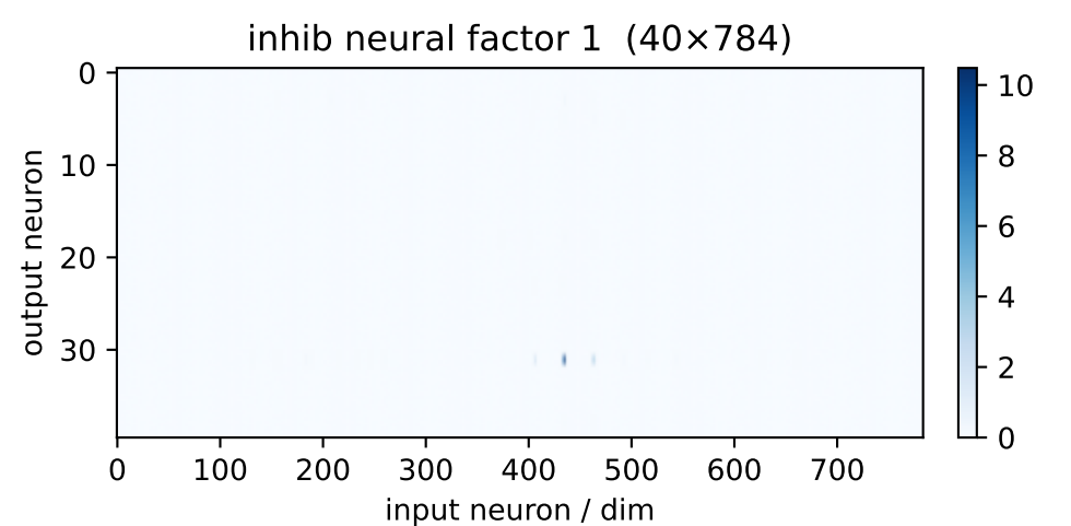
inh factor 1 \lambda=215.09 weighted avg
