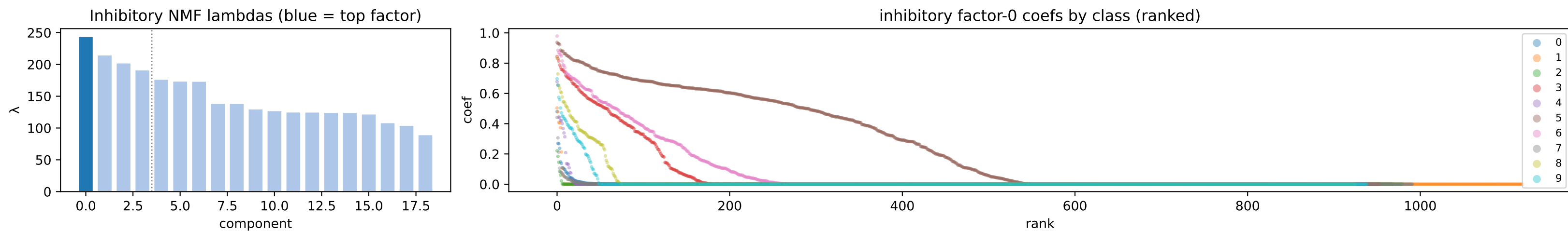
inh factor 0 \lambda=244.07 weighted avg
