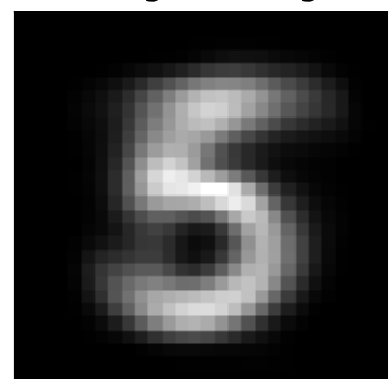
inh factor 2 \lambda=202.54 weighted avg
