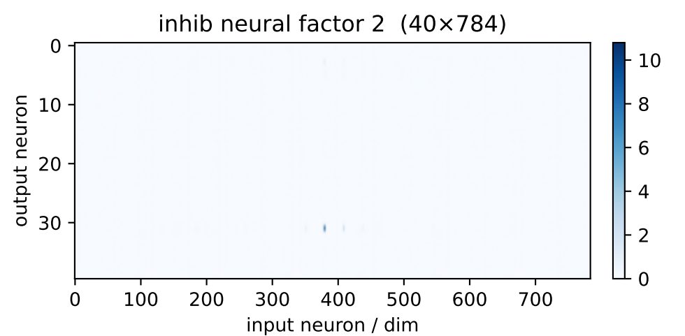
inh factor 2 \lambda=202.54 weighted avg
