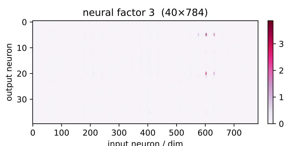
factor 3 \lambda=91.39 weighted avg
