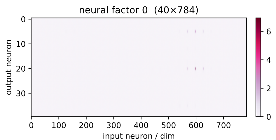
factor 0 \lambda=95.74 weighted avg
