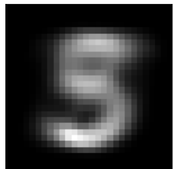
factor 1 \lambda=94.97 weighted avg
