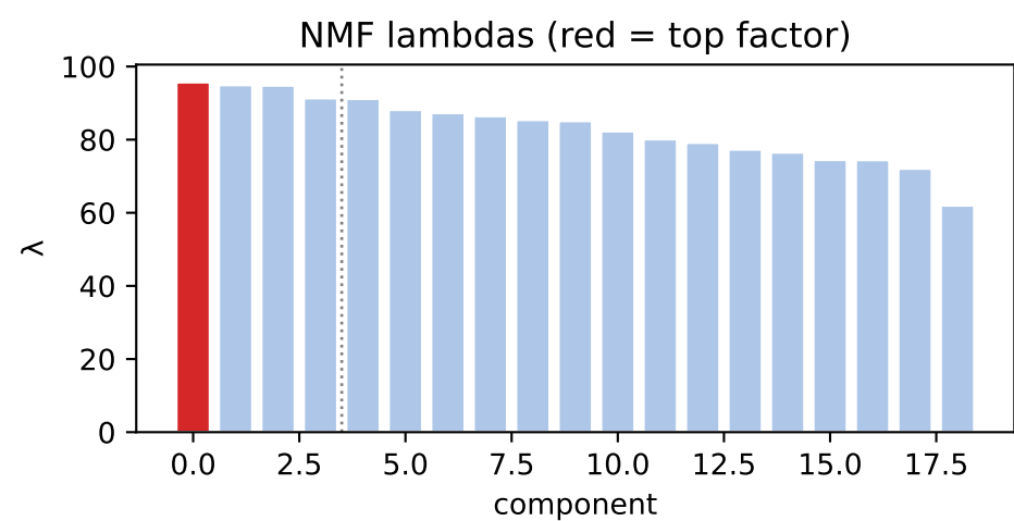
factor 0 \lambda=95.74 weighted avg
