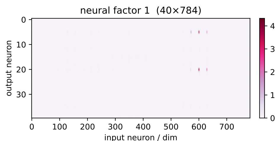
factor 1 \lambda=94.97 weighted avg
