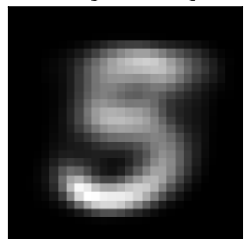
factor 0 \lambda=95.74 weighted avg
