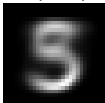
factor 2 \lambda=94.86 weighted avg
