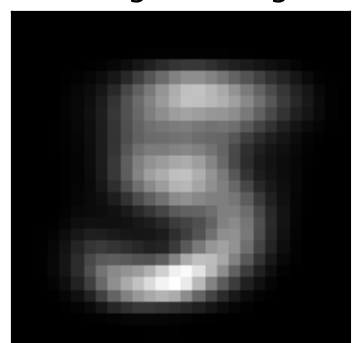
factor 3 \lambda=91.39 weighted avg
