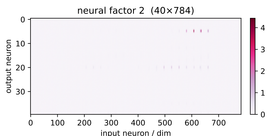
factor 2 \lambda=94.86 weighted avg
