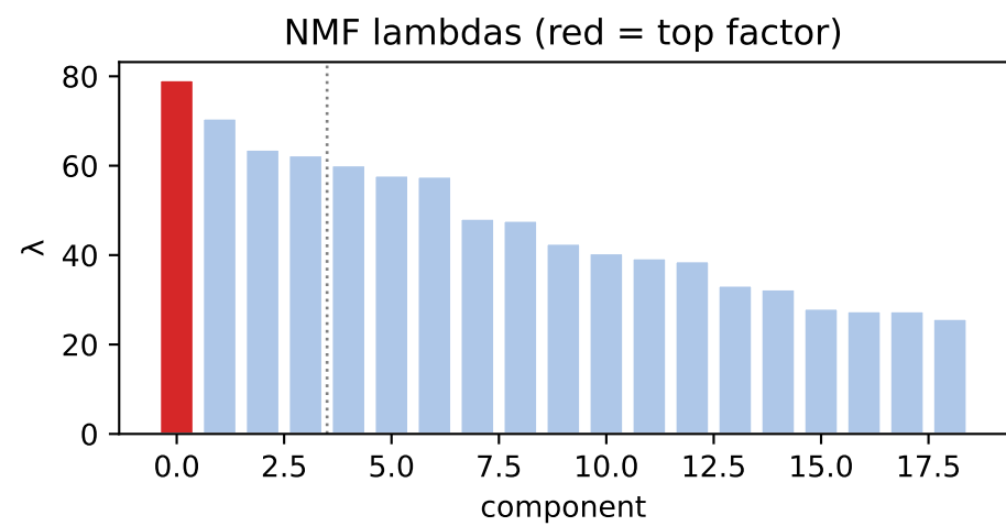
factor 0 \lambda=79.22 weighted avg
