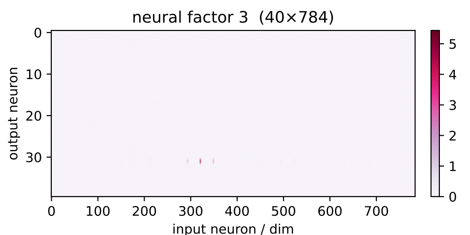
factor 3 \lambda=62.41 weighted avg
