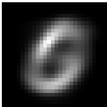
factor 0 \lambda=79.22 weighted avg
