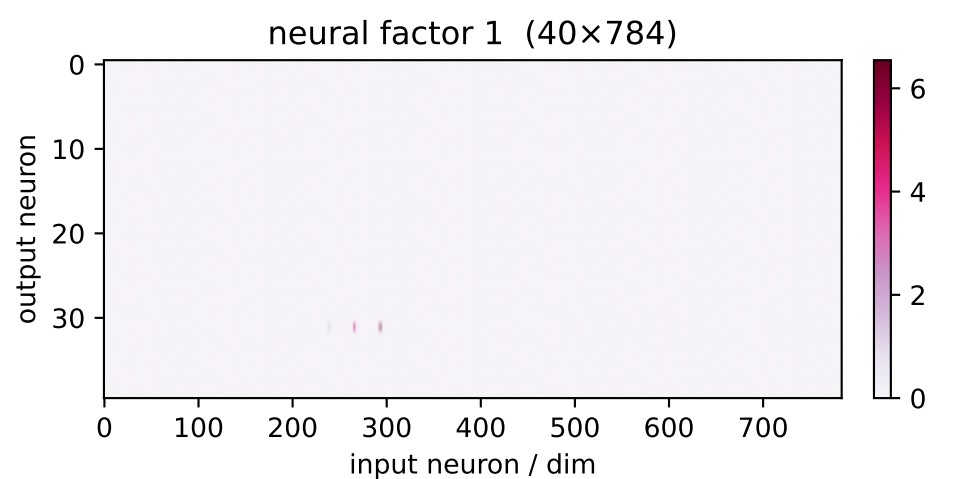
factor 1 \lambda=70.65 weighted avg
