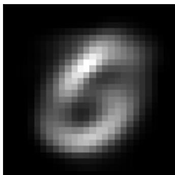
factor 1 \lambda=70.65 weighted avg
