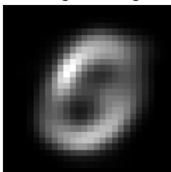
factor 2 \lambda=63.69 weighted avg
