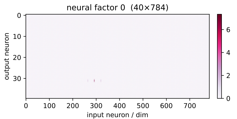
factor 0 \lambda=79.22 weighted avg
