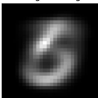
factor 3 \lambda=62.41 weighted avg
