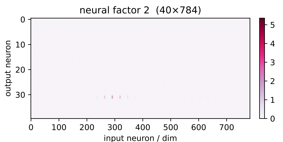
factor 2 \lambda=63.69 weighted avg
