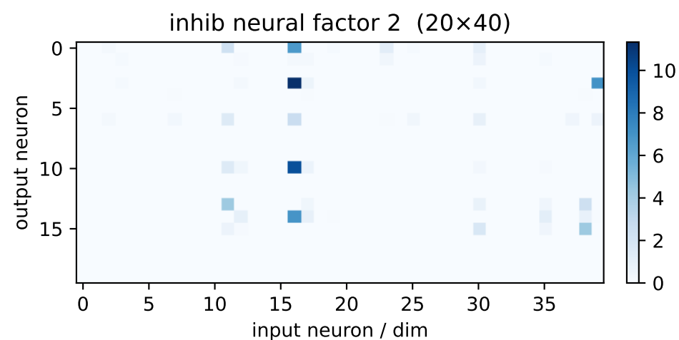
inh factor 2 \lambda=442.13 weighted avg
