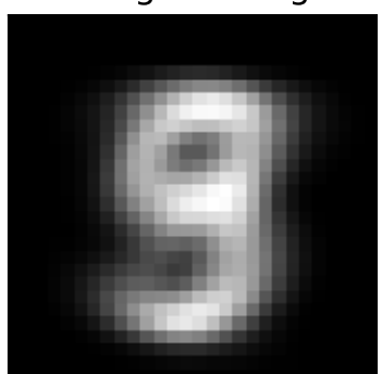
factor 2 \lambda=564.97 weighted avg
