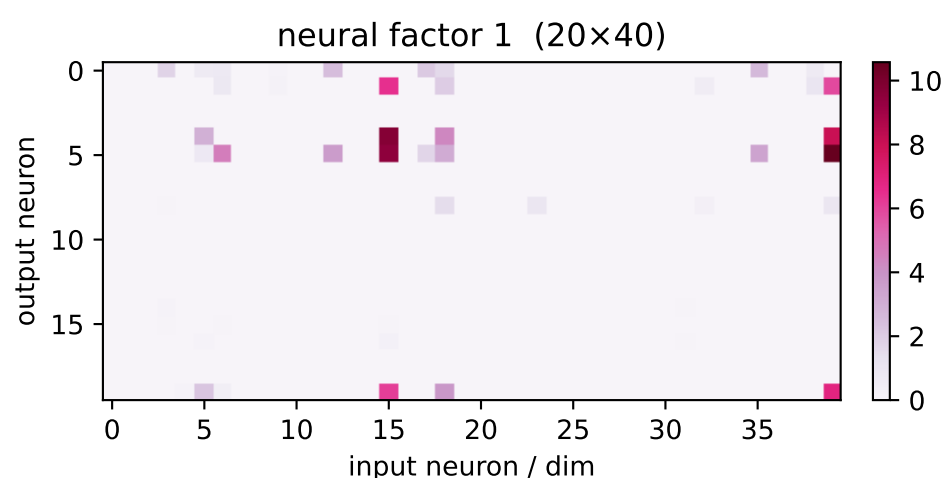
factor 1 \lambda=664.36 weighted avg
