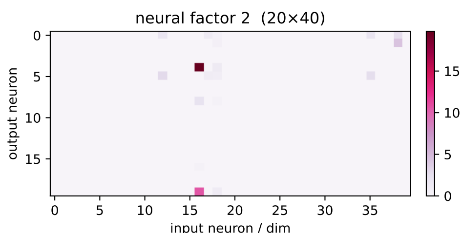
factor 2 \lambda=564.97 weighted avg
