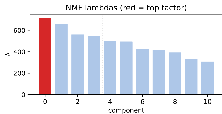
factor 0 \lambda=715.16 weighted avg
