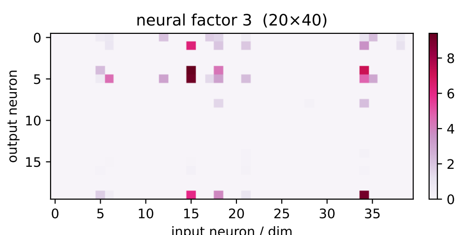
factor 3 \lambda=547.04 weighted avg
