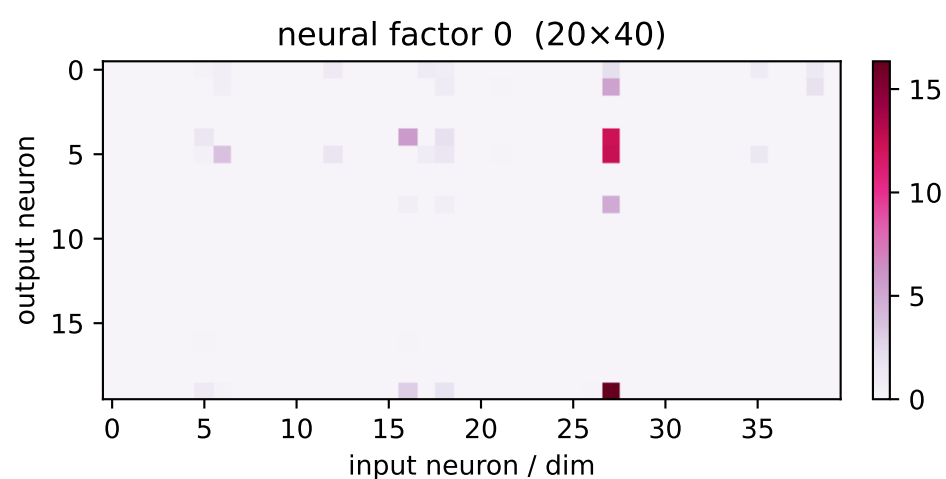
factor 0 \lambda=715.16 weighted avg
