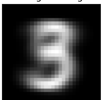
factor 3 \lambda=547.04 weighted avg
