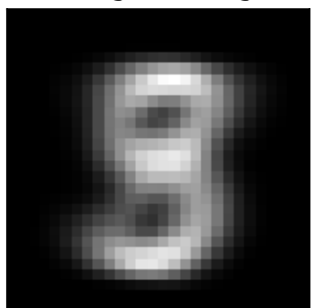
factor 0 \lambda=715.16 weighted avg
