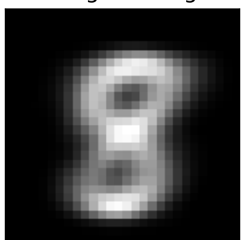
factor 1 \lambda=664.36 weighted avg
