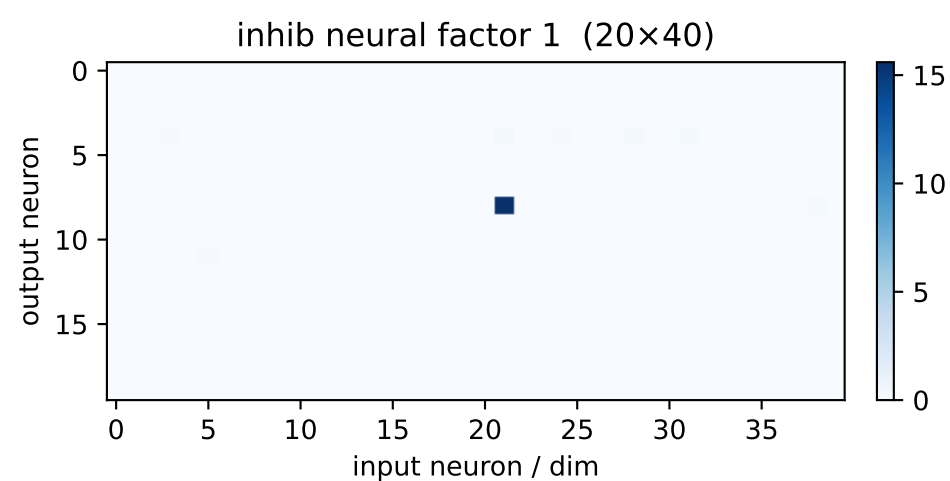
inh factor 1 \lambda=243.78 weighted avg
