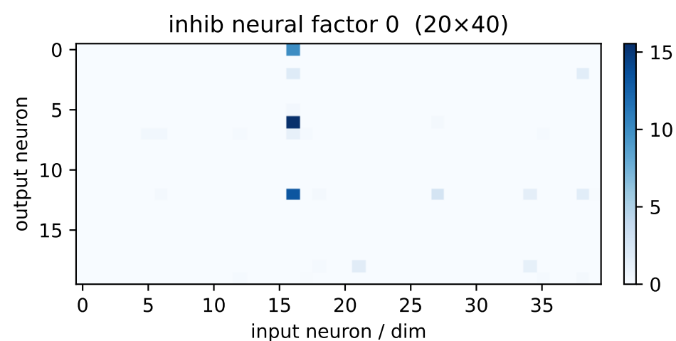
inh factor 0 \lambda=542.81 weighted avg
