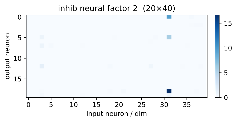
inh factor 2 \lambda=404.23 weighted avg
