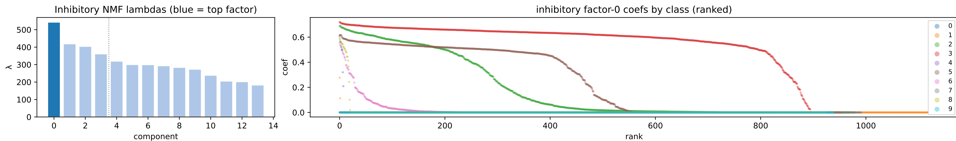
inh factor 0 \lambda=542.81 weighted avg
