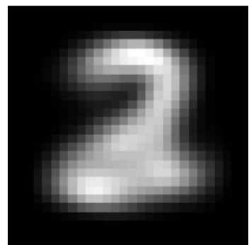
inh factor 1 \lambda=418.70 weighted avg
