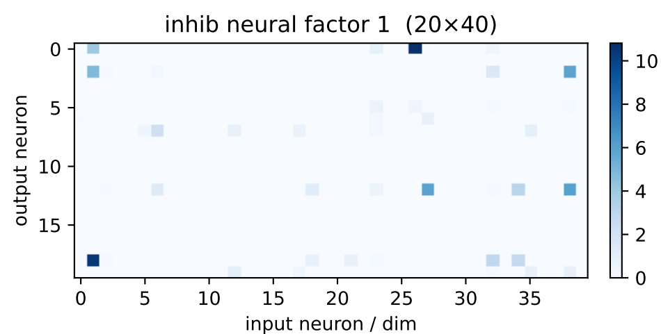
inh factor 1 \lambda=418.70 weighted avg
