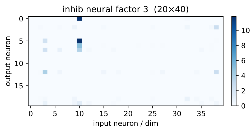
inh factor 3 \lambda=361.07 weighted avg
