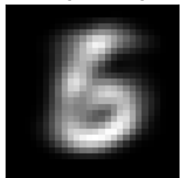
inh factor 3 \lambda=361.07 weighted avg
