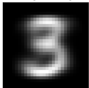
inh factor 0 \lambda=542.81 weighted avg
