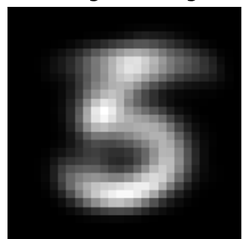
inh factor 2 \lambda=404.23 weighted avg
