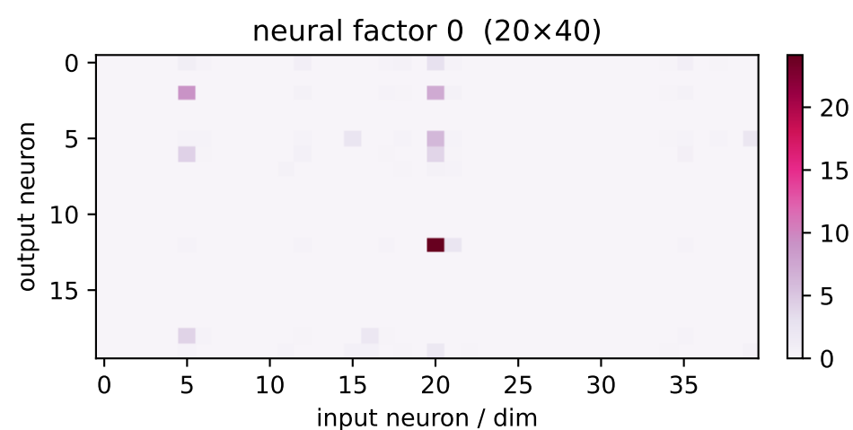
factor 0 \lambda=847.45 weighted avg
