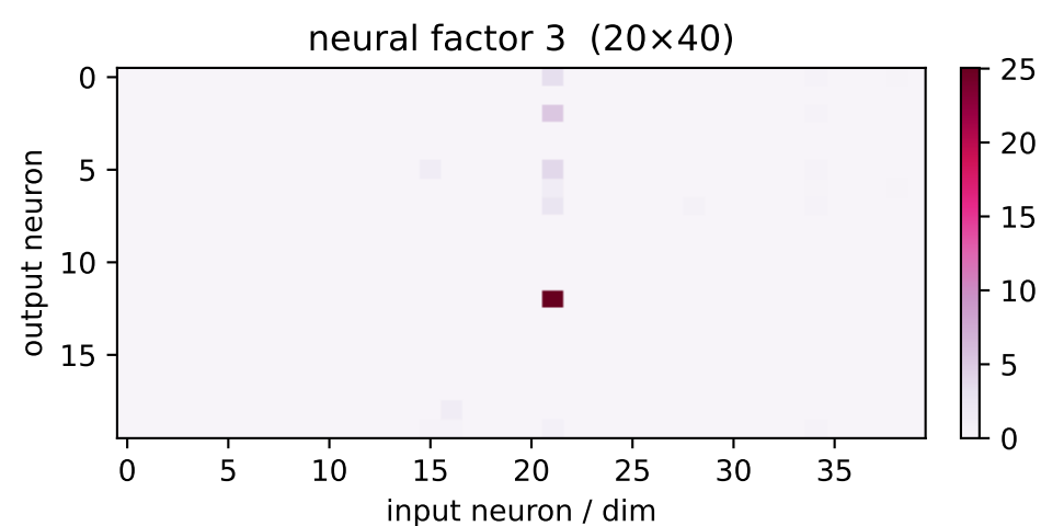
factor 3 \lambda=690.61 weighted avg
