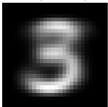
factor 3 \lambda=690.61 weighted avg
