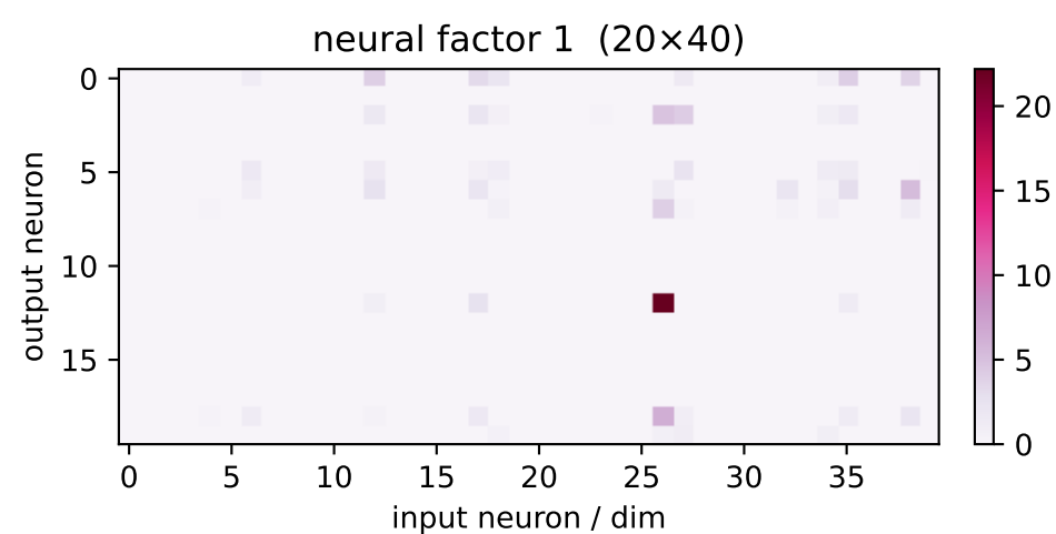
factor 1 \lambda=769.62 weighted avg
