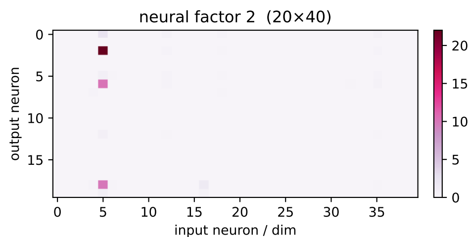
factor 2 \lambda=698.04 weighted avg
