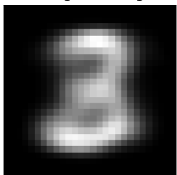
factor 2 \lambda=698.04 weighted avg
