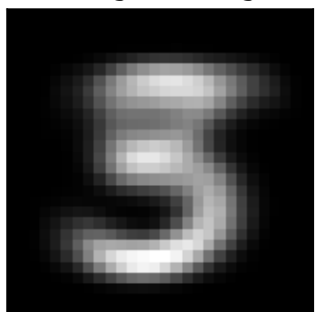
factor 0 \lambda=847.45 weighted avg
