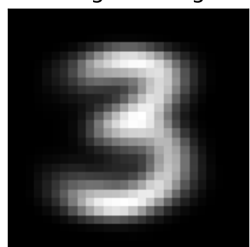
inh factor 1 \lambda=544.05 weighted avg
