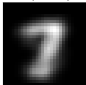
inh factor 2 \lambda=430.84 weighted avg
