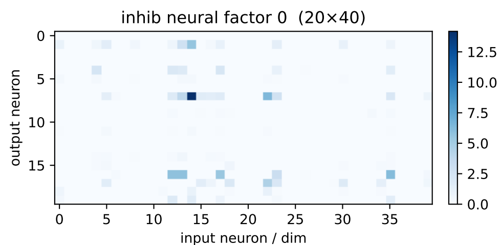
inh factor 0 \lambda=551.60 weighted avg
