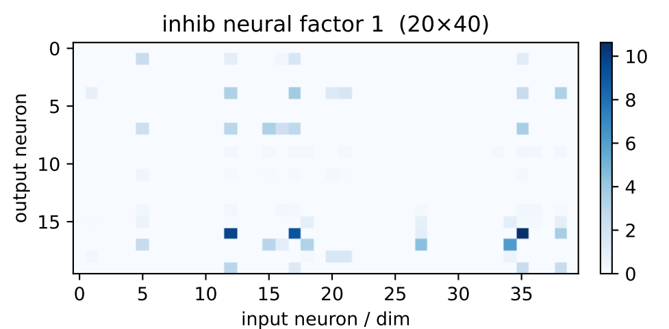
inh factor 1 \lambda=544.05 weighted avg
