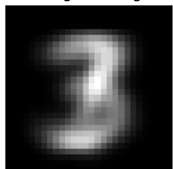
inh factor 3 \lambda=415.86 weighted avg
