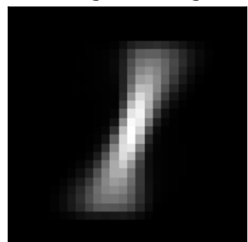
inh factor 0 \lambda=551.60 weighted avg
