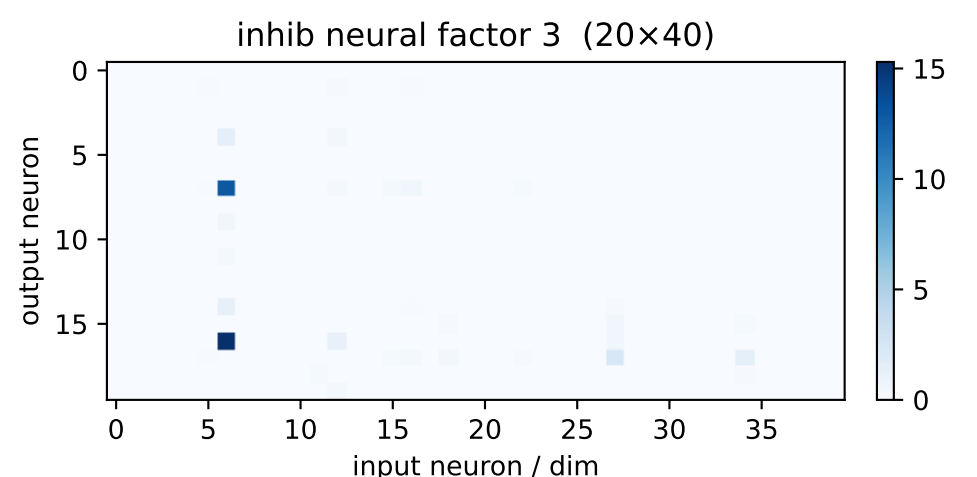
inh factor 3 \lambda=415.86 weighted avg
