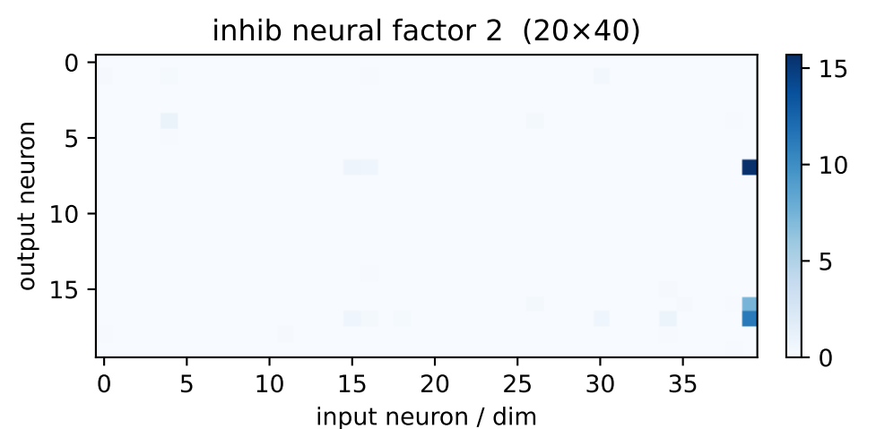
inh factor 2 \lambda=430.84 weighted avg
