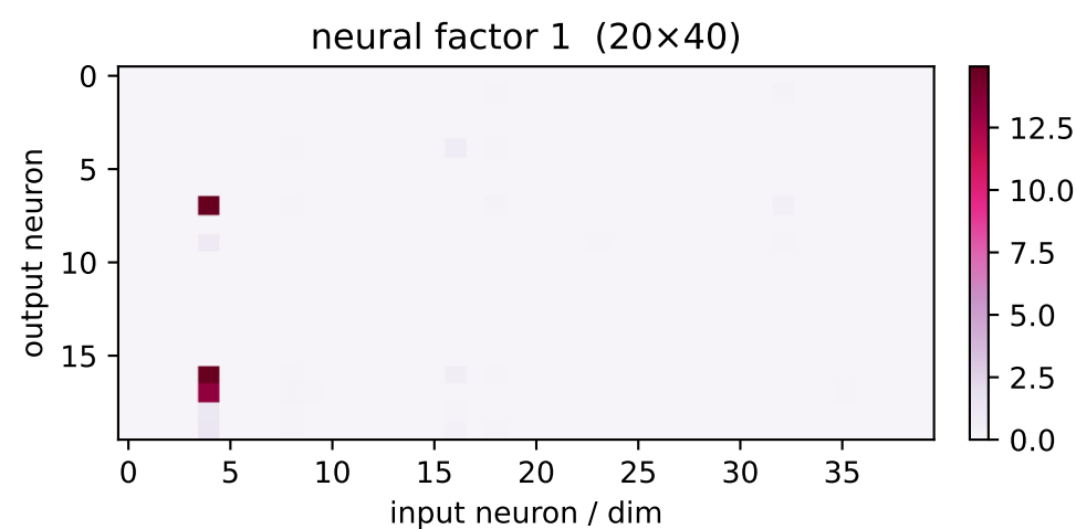
factor 1 \lambda=628.64 weighted avg
