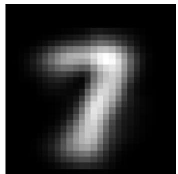
factor 1 \lambda=628.64 weighted avg
