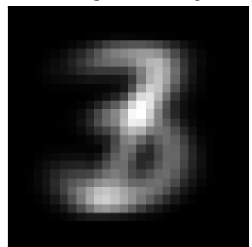
factor 3 \lambda=538.04 weighted avg
