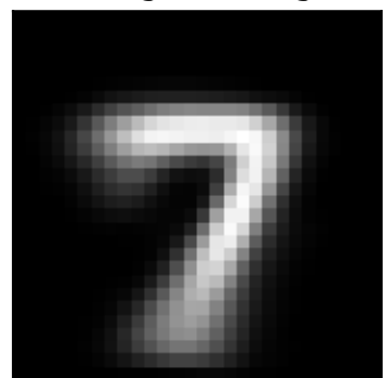
factor 0 \lambda=713.13 weighted avg
