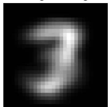
factor 2 \lambda=543.87 weighted avg
