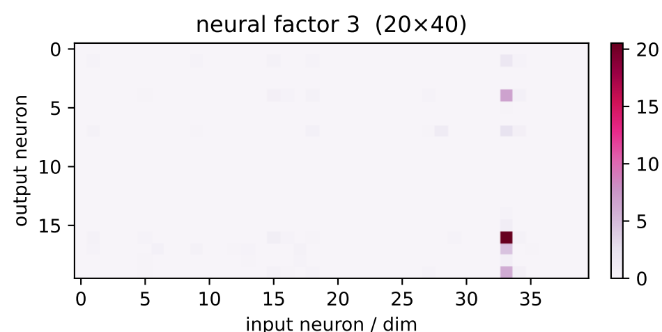
factor 3 \lambda=538.04 weighted avg
