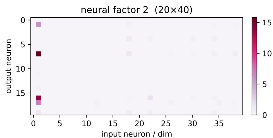
factor 2 \lambda=543.87 weighted avg
