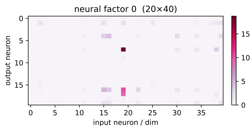
factor 0 \lambda=713.13 weighted avg
