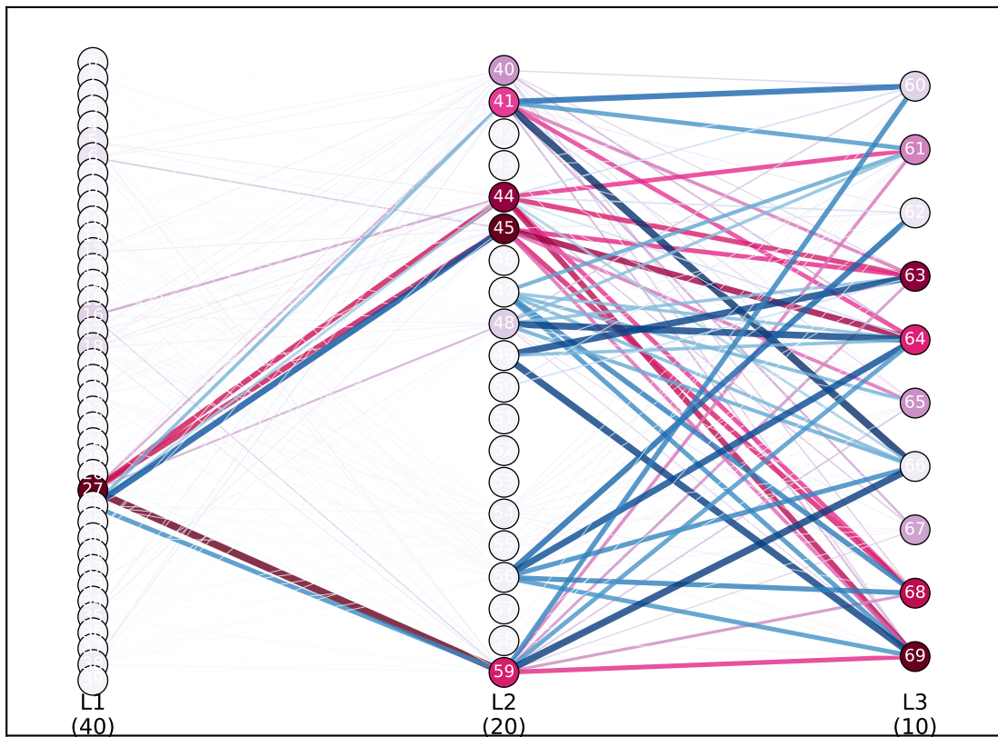
Factor Trace — Network Scaffold [path: F4→F0] (NMF factor at each layer, traced backwards from output)
