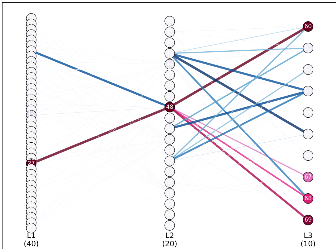
Factor Trace — Network Scaffold [path: F5→F0] (NMF factor at each layer, traced backwards from output)
