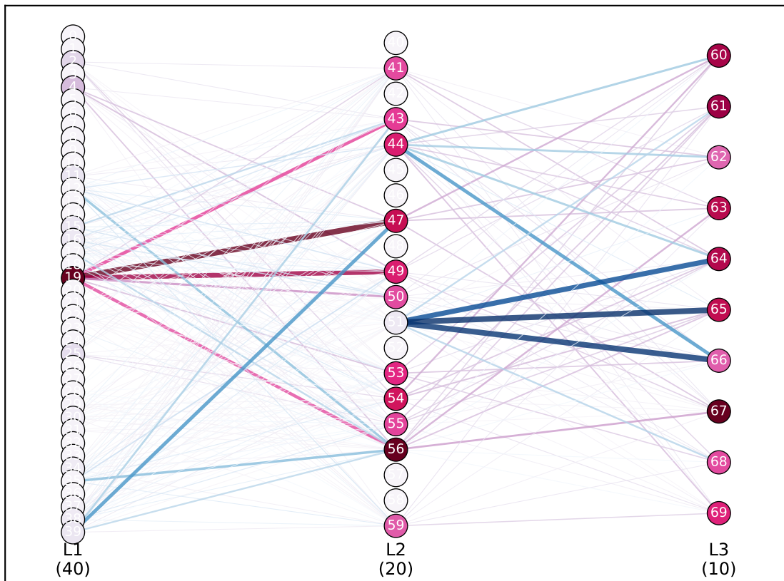
Factor Trace — Network Scaffold [path: F8→F0] (NMF factor at each layer, traced backwards from output)
