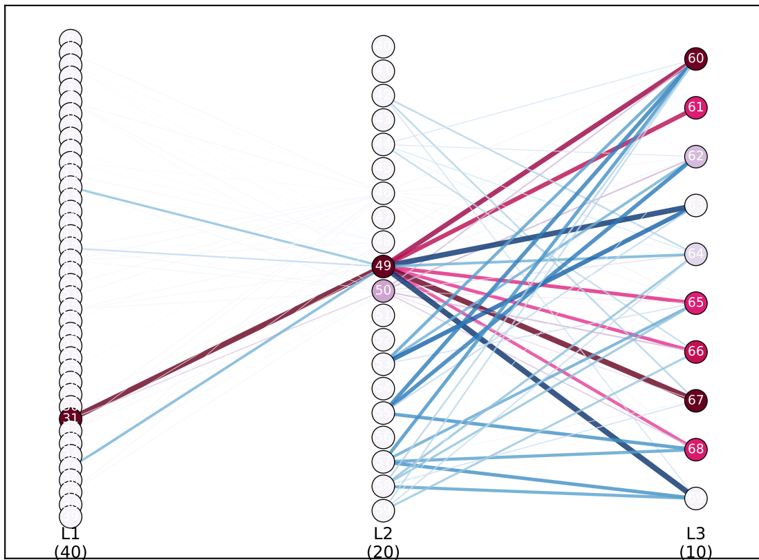
Factor Trace — Network Scaffold [path: F9→F0] (NMF factor at each layer, traced backwards from output)
