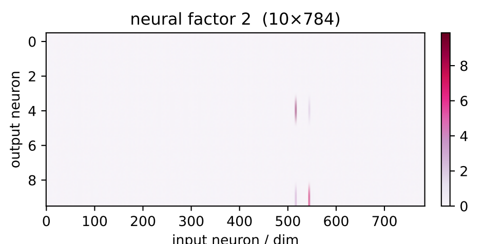
factor 2 \lambda=266.58 weighted avg
