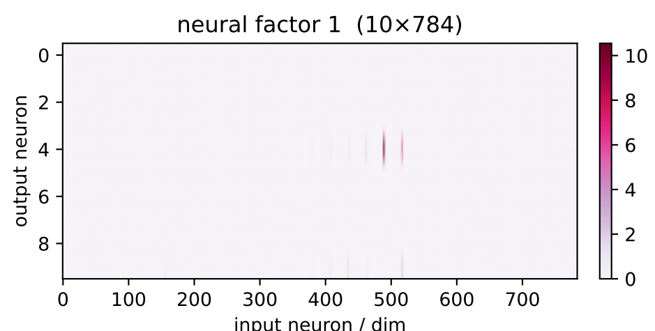
factor 1 \lambda=278.59 weighted avg
