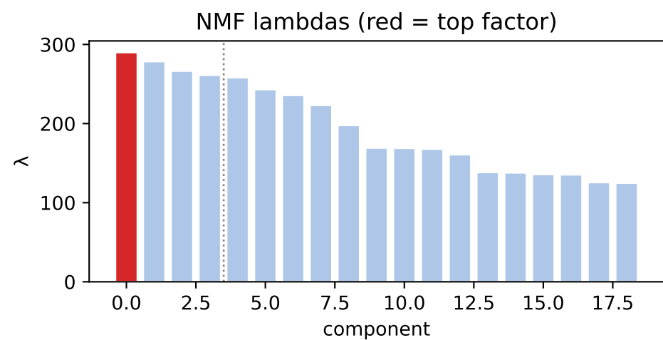
factor 0 \lambda=289.96 weighted avg
