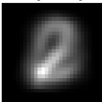
factor 2 \lambda=266.58 weighted avg
