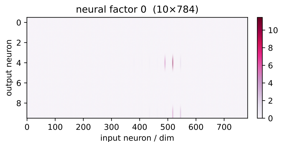
factor 0 \lambda=289.96 weighted avg
