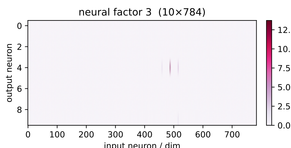
factor 3 \lambda=261.27 weighted avg
