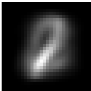
factor 0 \lambda=289.96 weighted avg
