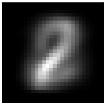
factor 1 \lambda=278.59 weighted avg
