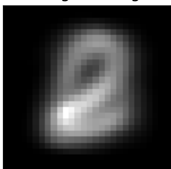
factor 3 \lambda=261.27 weighted avg
