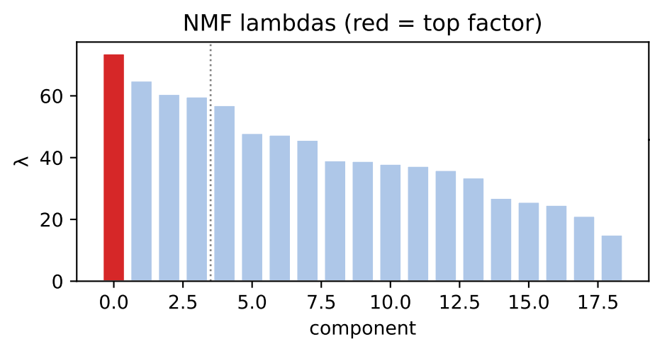
factor 0 \lambda=73.73 weighted avg
