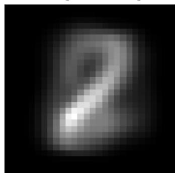
factor 3 \lambda=59.78 weighted avg
