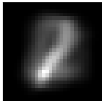
factor 1 \lambda=64.94 weighted avg
