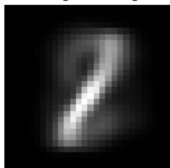
factor 2 \lambda=60.61 weighted avg
