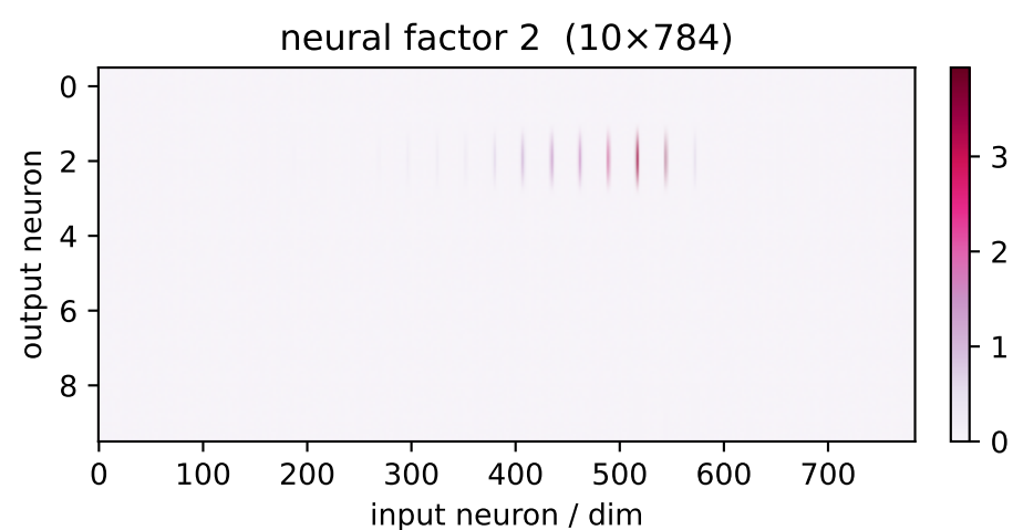
factor 2 \lambda=60.61 weighted avg
