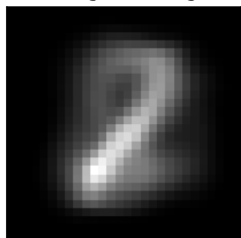
factor 0 \lambda=73.73 weighted avg
