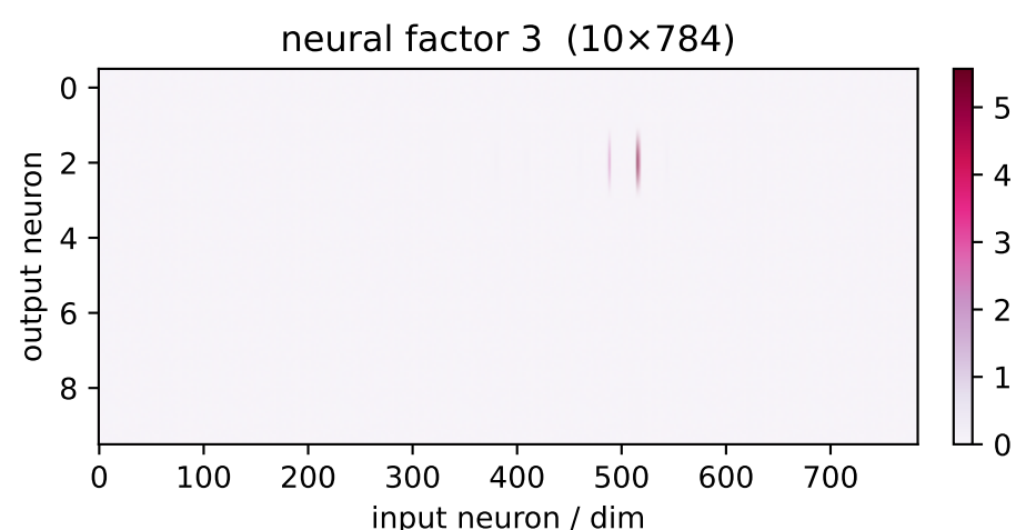
factor 3 \lambda=59.78 weighted avg
