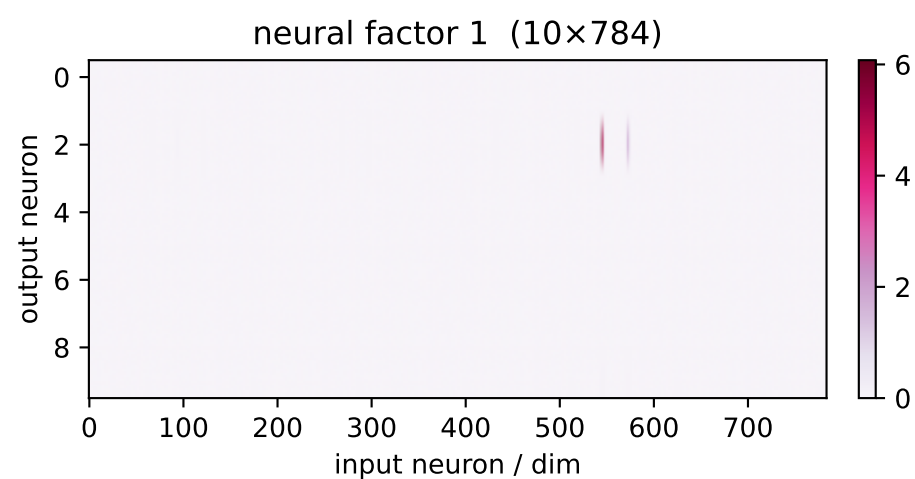
factor 1 \lambda=64.94 weighted avg
