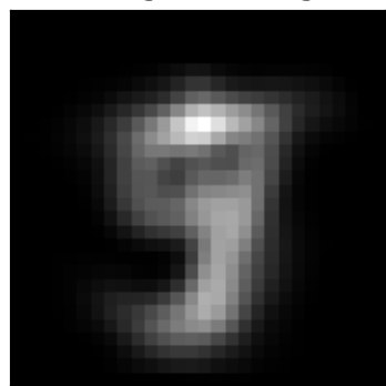
factor 3 \lambda=42.56 weighted avg
