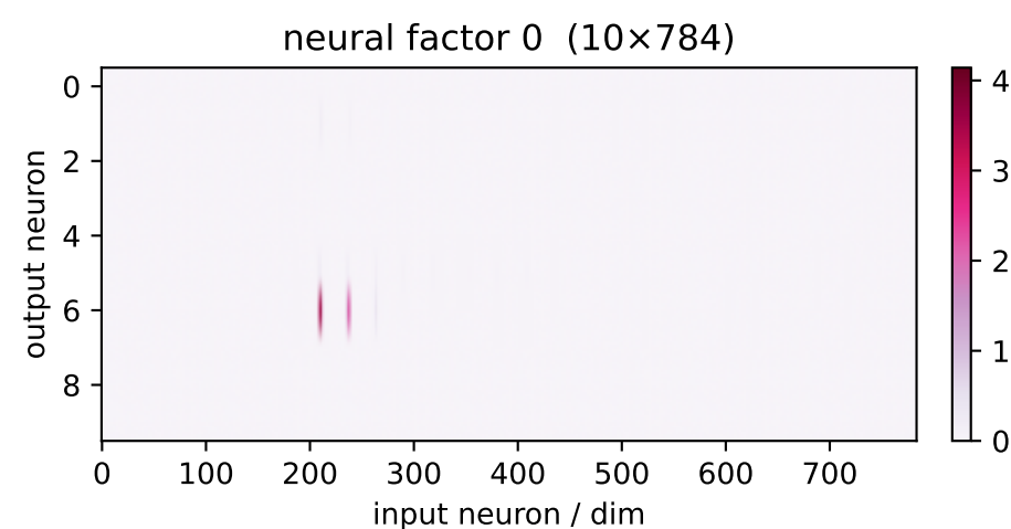
factor 0 \lambda=51.02 weighted avg
