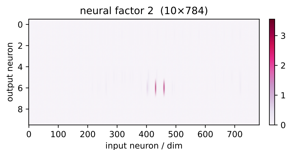
factor 2 \lambda=42.66 weighted avg
