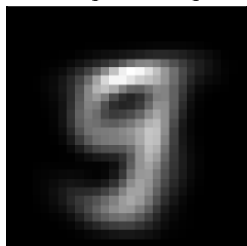
factor 0 \lambda=51.02 weighted avg
