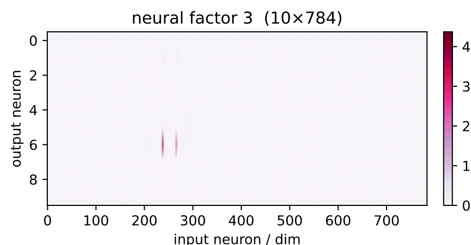
factor 3 \lambda=42.56 weighted avg
