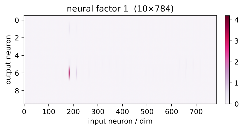
factor 1 \lambda=44.68 weighted avg
