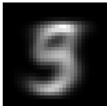
factor 1 \lambda=44.68 weighted avg
