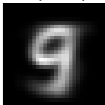
factor 2 \lambda=42.66 weighted avg
