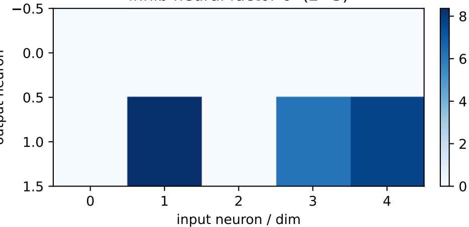
inhib neural factor 0 (2×5)
