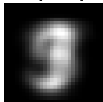
inh factor 1 \lambda=147.81 weighted avg
