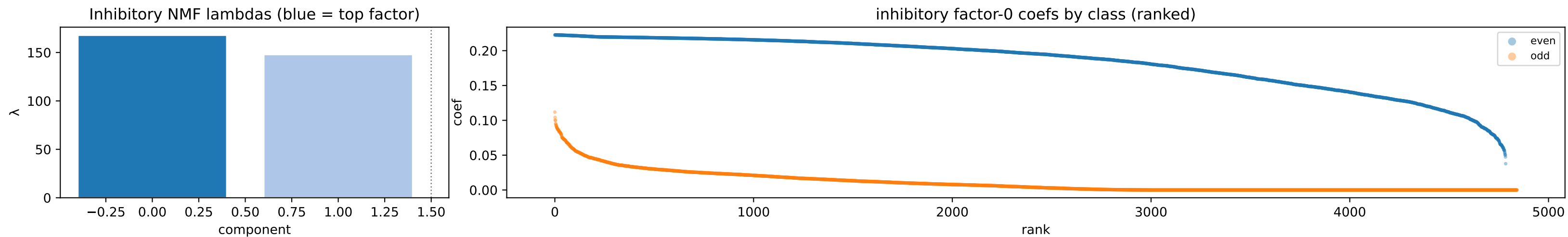
inh factor 0 \lambda=167.76 weighted avg
