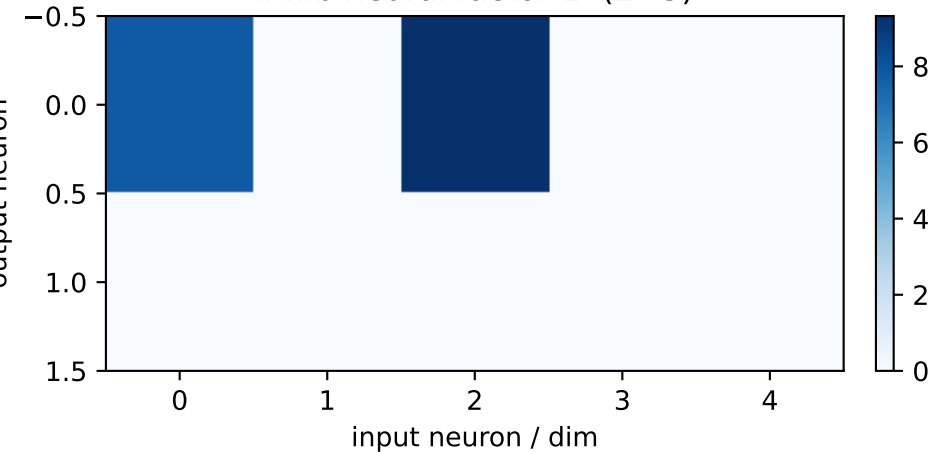
inhib neural factor 1 (2×5)
