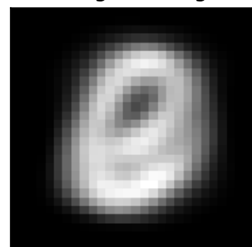
inh factor 0 \lambda=167.76 weighted avg
