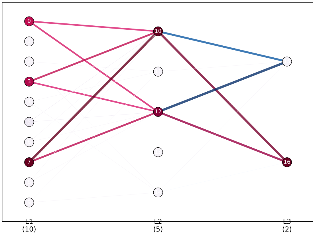
Factor Trace — Network Scaffold [path: F1→F3] (NMF factor at each layer, traced backwards from output)
