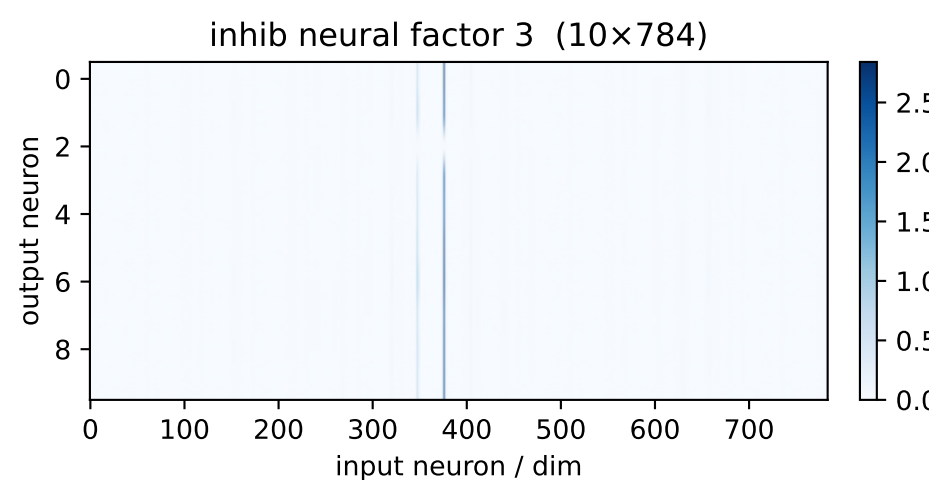
inh factor 3 \lambda=78.33 weighted avg
