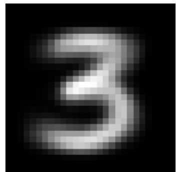
inh factor 2 \lambda=89.43 weighted avg
