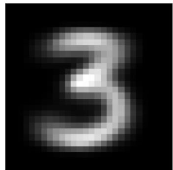
inh factor 3 \lambda=78.33 weighted avg
