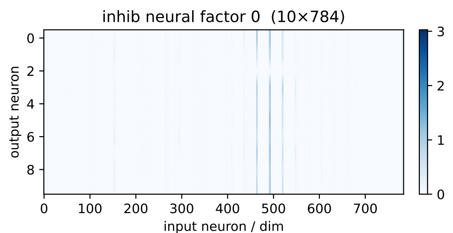
inh factor 0 \lambda=113.90 weighted avg
