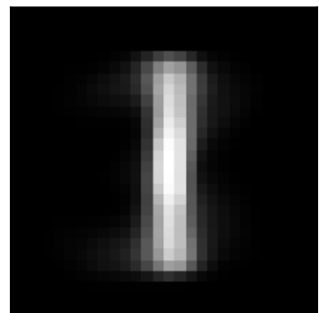
inh factor 0 \lambda=113.90 weighted avg
