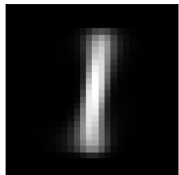
inh factor 1 \lambda=92.52 weighted avg
