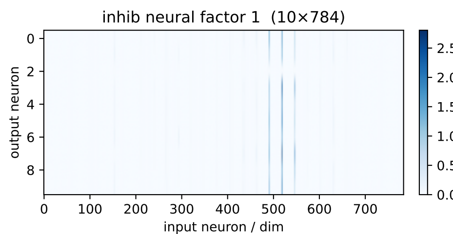
inh factor 1 \lambda=92.52 weighted avg
