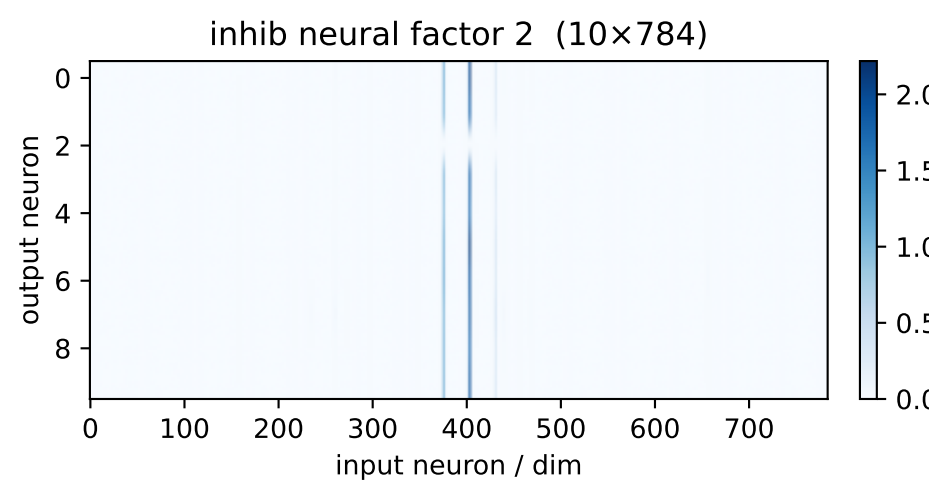
inh factor 2 \lambda=89.43 weighted avg
