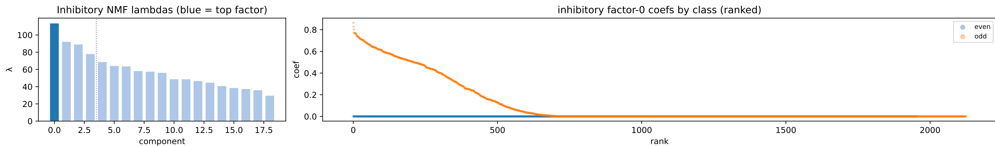
inh factor 0 \lambda=113.90 weighted avg
