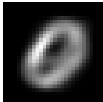
factor 2 \lambda=29.90 weighted avg
