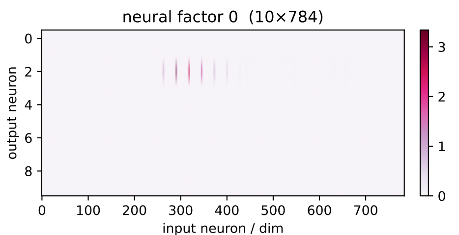
factor 0 \lambda=35.66 weighted avg
