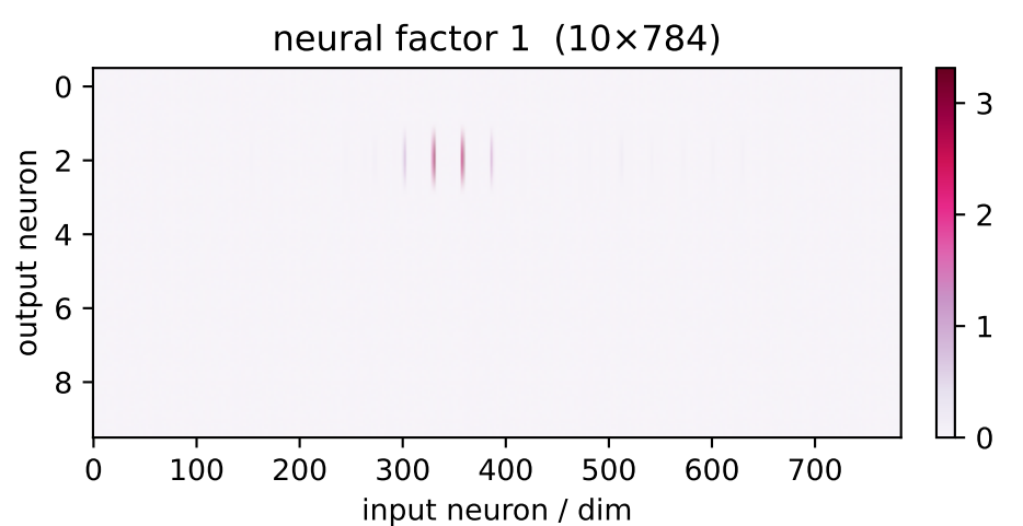
factor 1 \lambda=32.19 weighted avg
