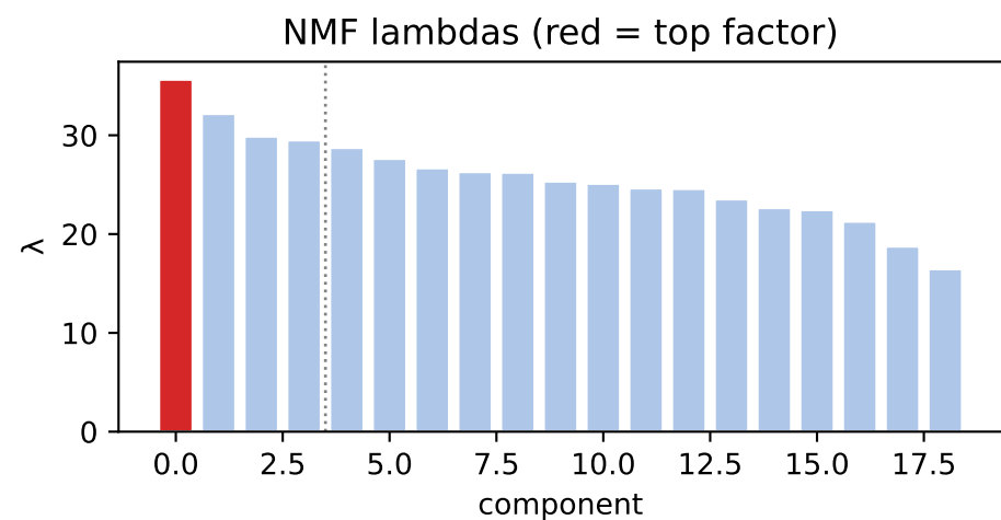
factor 0 \lambda=35.66 weighted avg
