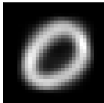
factor 1 \lambda=32.19 weighted avg
