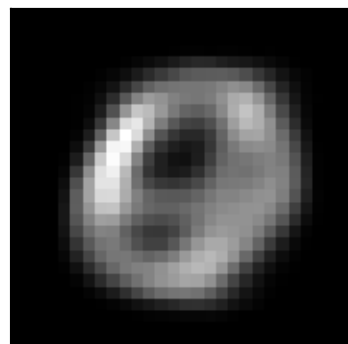
factor 3 \lambda=29.52 weighted avg
