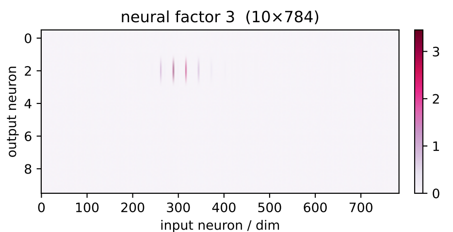
factor 3 \lambda=29.52 weighted avg
