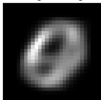
factor 0 \lambda=35.66 weighted avg
