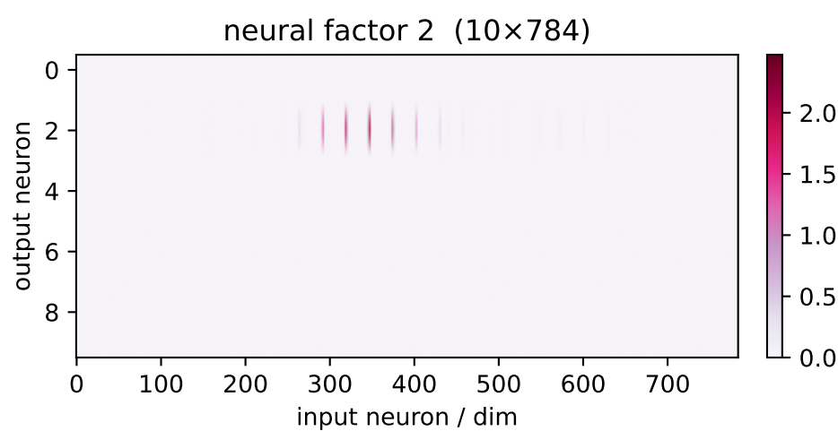
factor 2 \lambda=29.90 weighted avg
