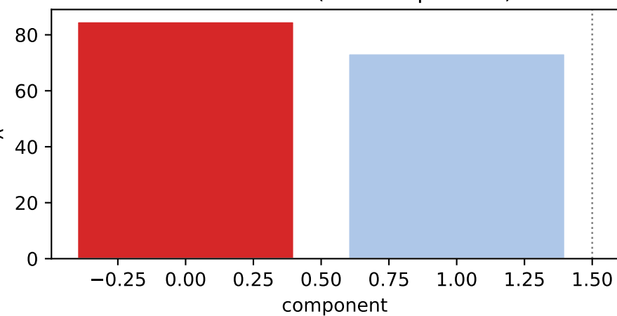
factor 0 \lambda=84.81 weighted avg
