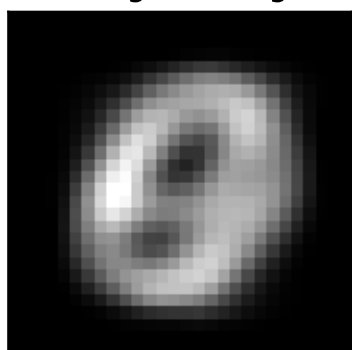
factor 1 \lambda=73.35 weighted avg
