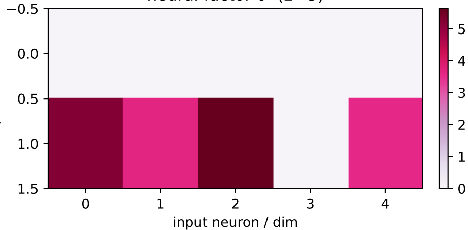
neural factor 0 (2×5)
