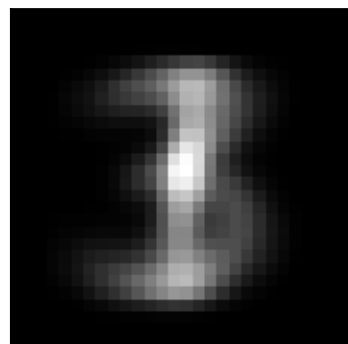
factor 1 \lambda=30.05 weighted avg
