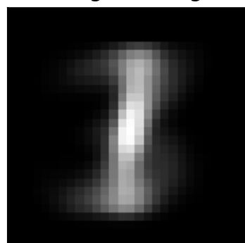
factor 0 \lambda=34.47 weighted avg
