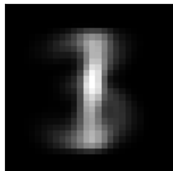
factor 3 \lambda=25.04 weighted avg
