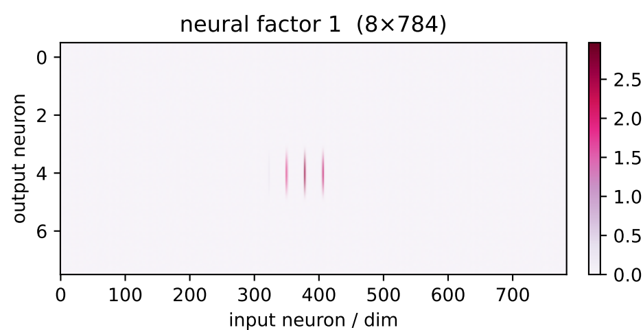
factor 1 \lambda=30.05 weighted avg
