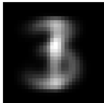
factor 2 \lambda=27.82 weighted avg
