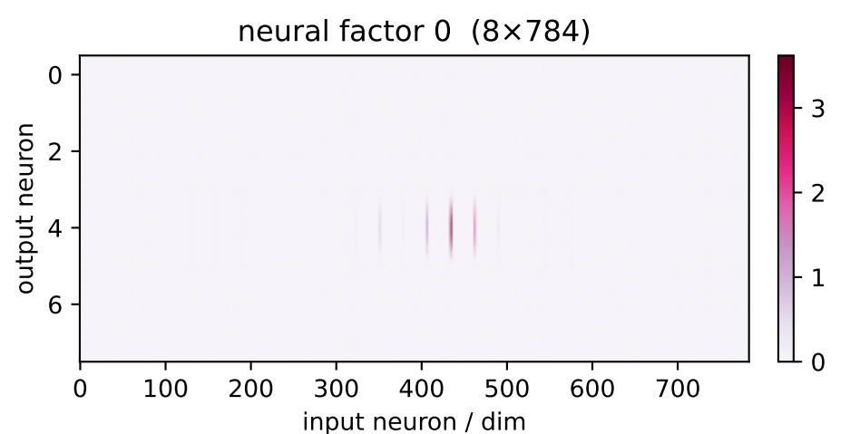
factor 0 \lambda=34.47 weighted avg
