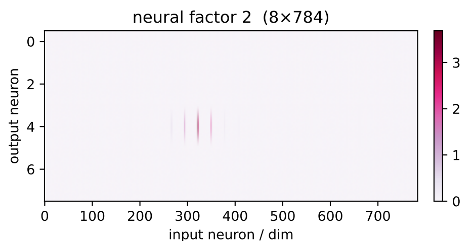
factor 2 \lambda=27.82 weighted avg
