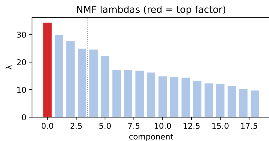
factor 0 \lambda=34.47 weighted avg
