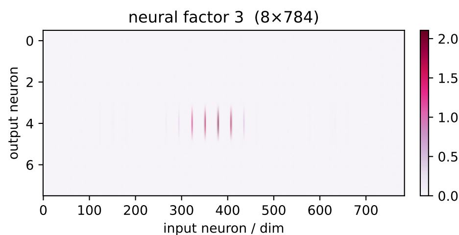
factor 3 \lambda=25.04 weighted avg
