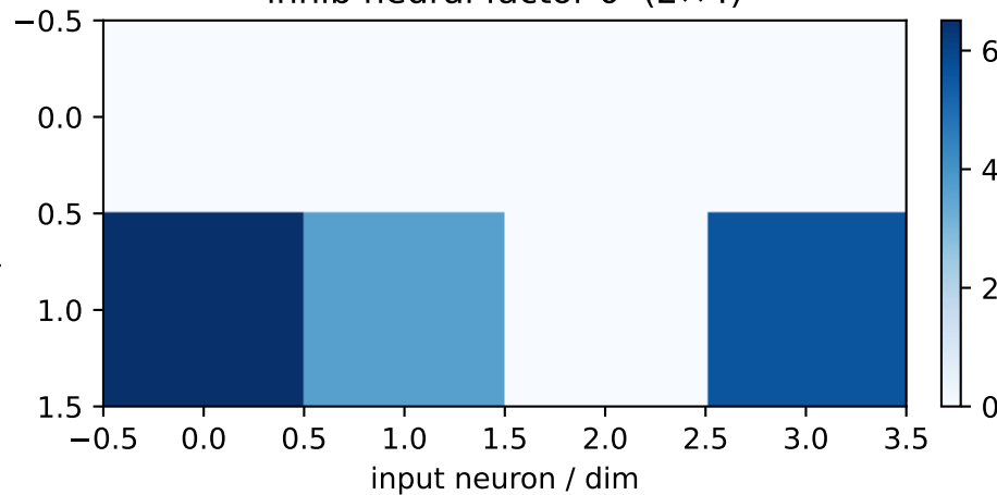
inhib neural factor 0 (2x4)
