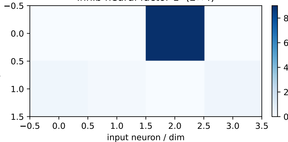
inhib neural factor 1 (2x4)
