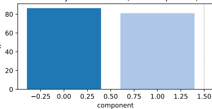
inh factor 0 \lambda=86.81 weighted avg
