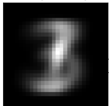
inh factor 1 \lambda=81.45 weighted avg
