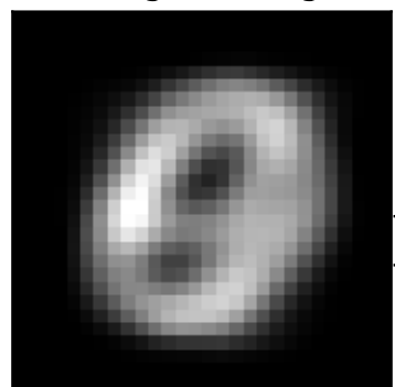
inh factor 0 \lambda=86.81 weighted avg
