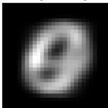
factor 0 \lambda=84.47 weighted avg
