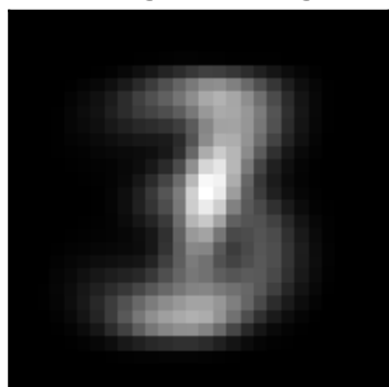
factor 1 \lambda=73.56 weighted avg
