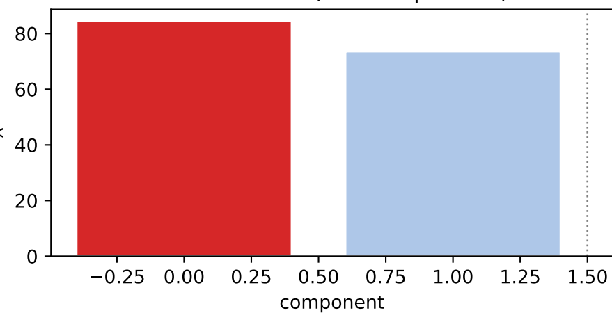
factor 0 \lambda=84.47 weighted avg
