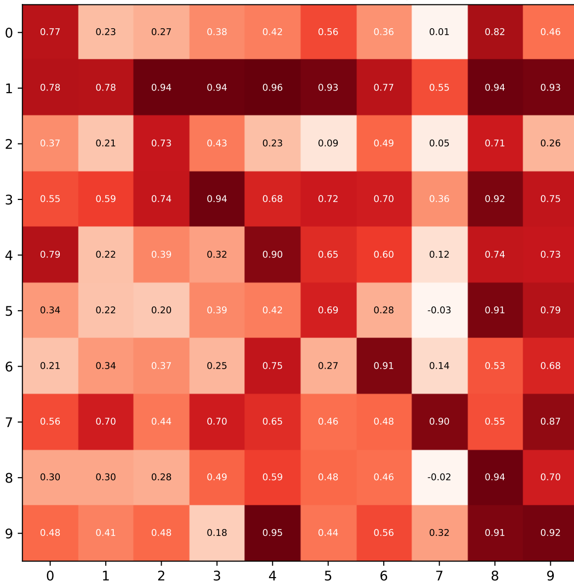
Specificity Matrix (pct=90) Diagonal = target; off-diagonal = bystander
