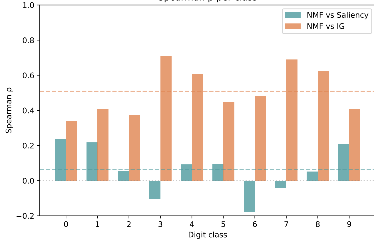
NMF vs Gradient Attribution Spearman \rho per class
