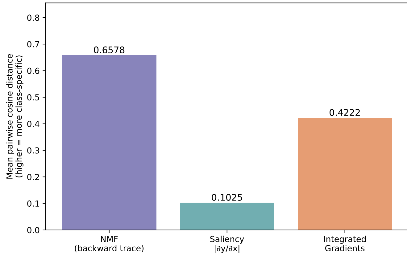
Class Discriminability of Attribution Maps
