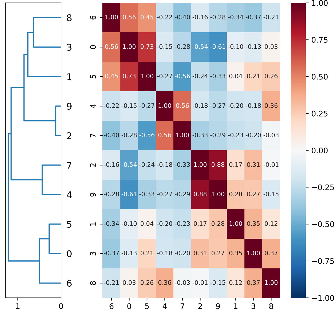
Stimulus Loading Spearman \rho (L2 child)
