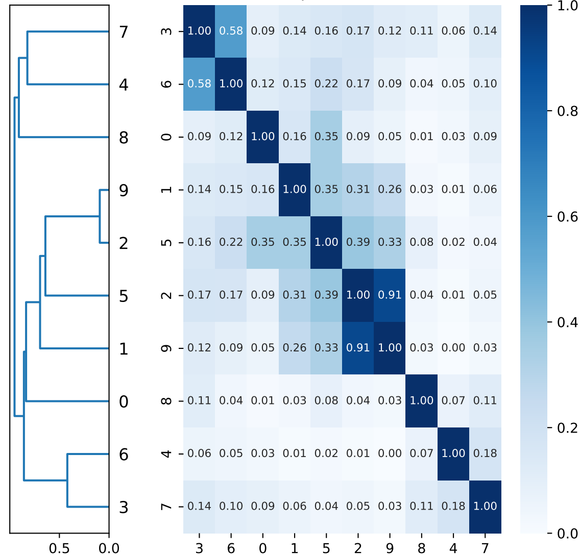
L1 Circuit Cosine Sim (pixel-level)
