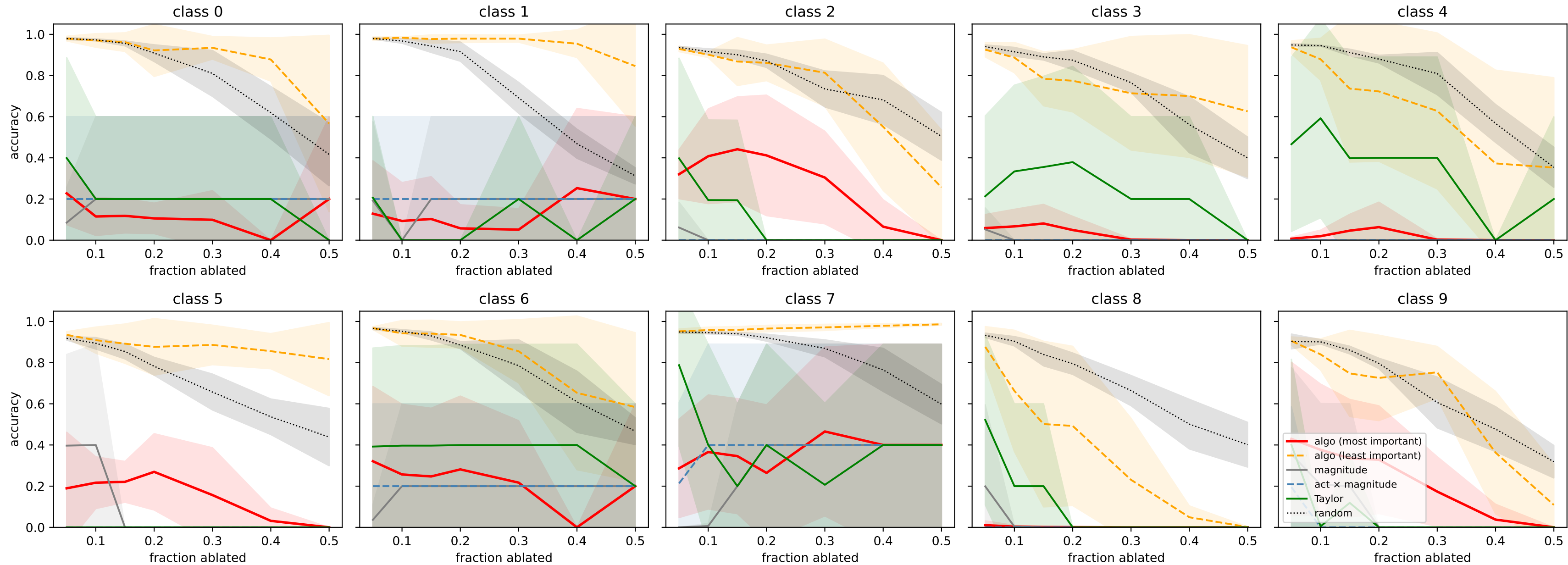
Per-class accuracy after ablating top-f fraction of weights
