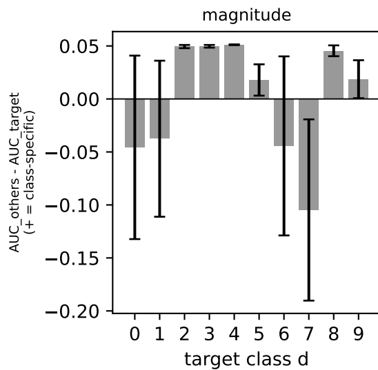
Within-run AUC gap algo_bottom: positive = target spared; all others: positive = class-specific damage
