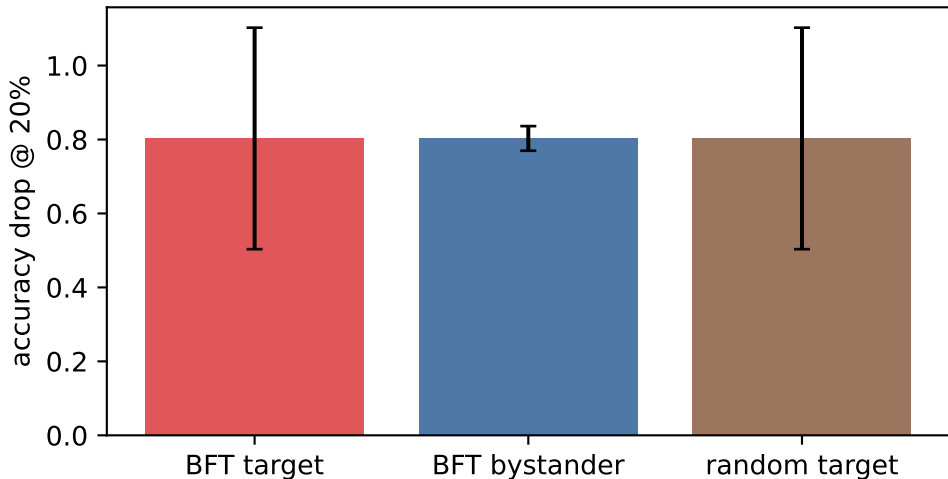
Circuit ablation — cnn_cifar (generic filter-level proxy; Wilcoxon p=0.084 )
