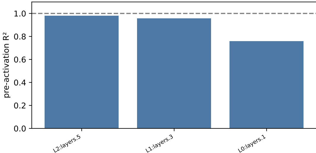
FU2 fc-node reconstruction — mlp_even_odd
