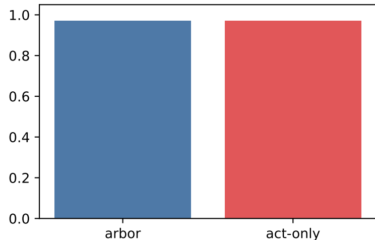
fingerprint kNN
