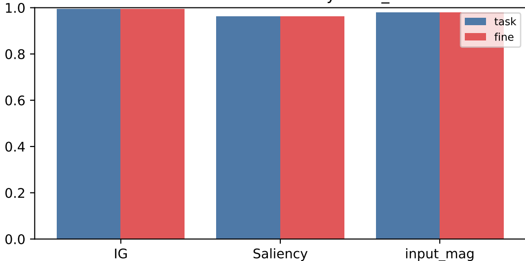
attribution discriminability — vit_mnist
