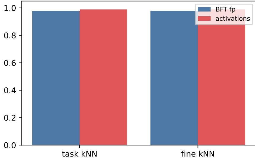
class separability
