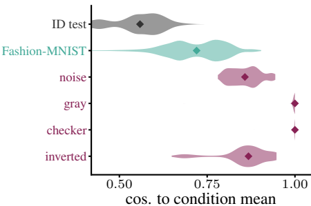
(c) NNLS round-trip
