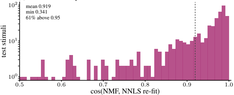
(c) NNLS round-trip
