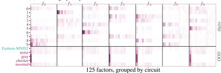
(b) mean fingerprint per condition
