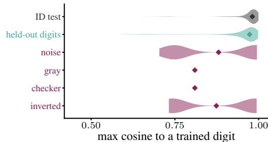
(e) distance to the trained digits
