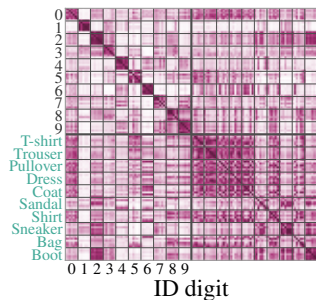
(c) digits vs Fashion-MNIST
