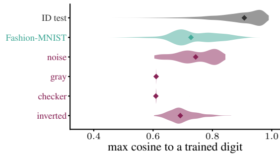
(e) distance to the trained digits
