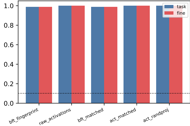
kNN accuracy (dotted = shuffled-label null)
