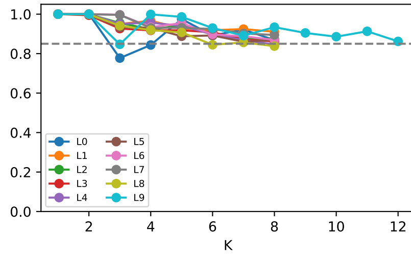
NMF stability
