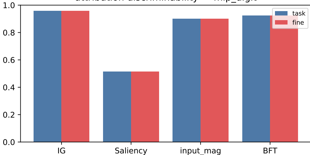
attribution discriminability — mlp_digit
