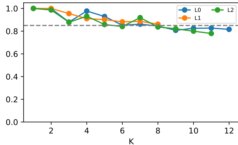
NMF stability
