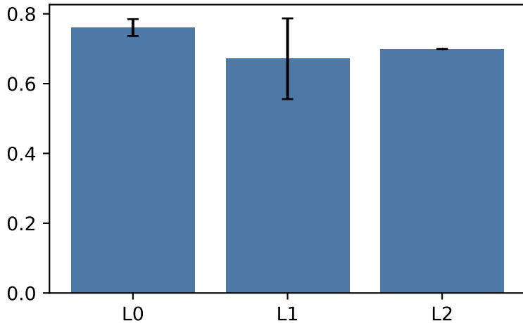
pre-activation R 2
