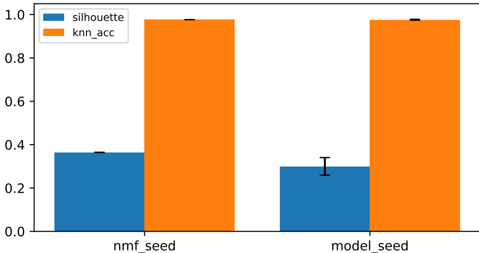
seed variability — mlp_digit
