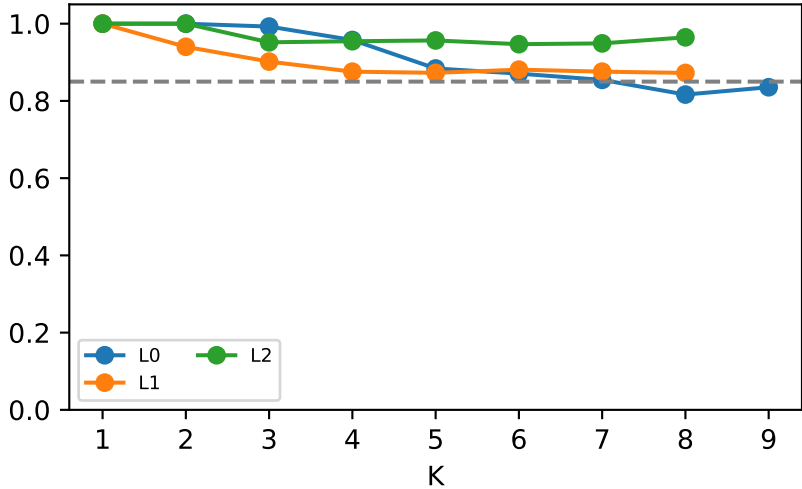
NMF stability
