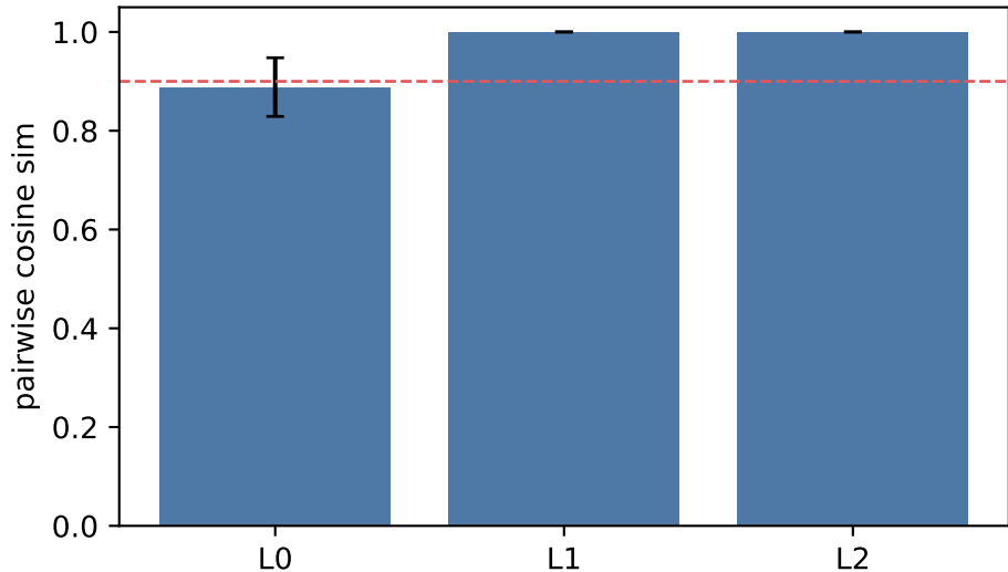
NMF stability — mlp_even_odd
