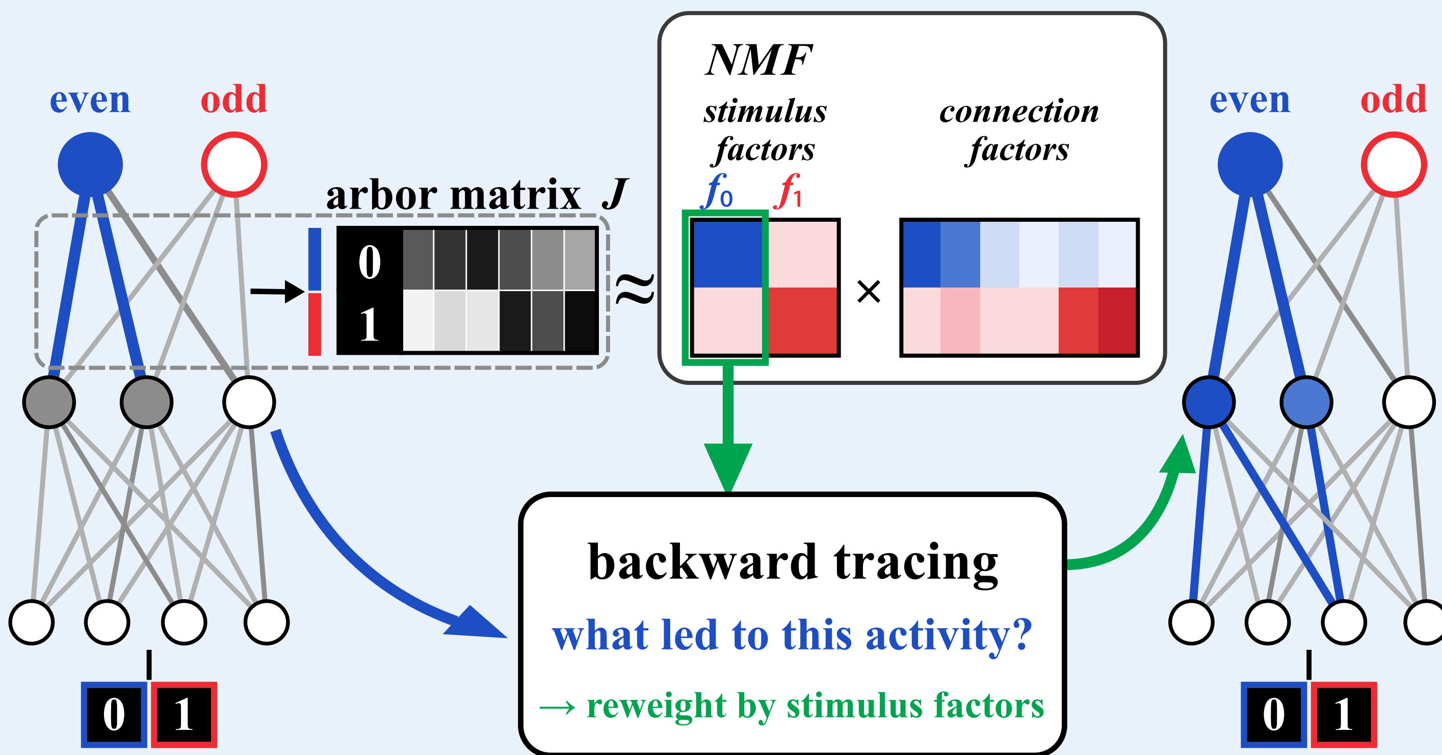
(b) Backward Factor Tracing (BFT)
