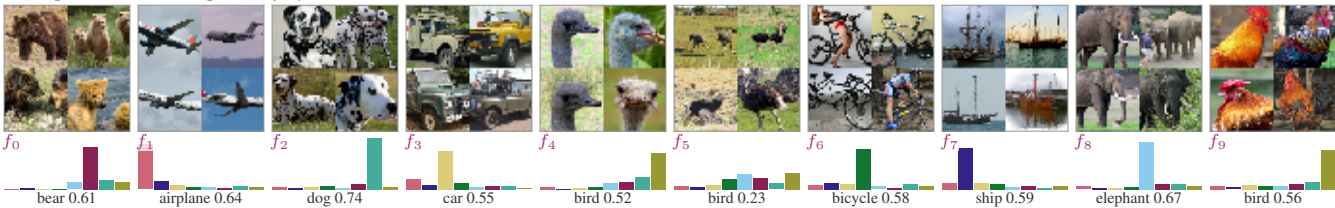
(b) traceback to L_9
