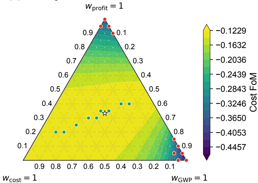
(a) Cost figure of merit
