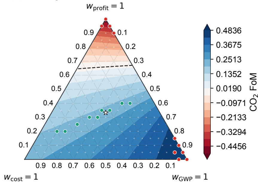
(b) CO 2 figure of merit
